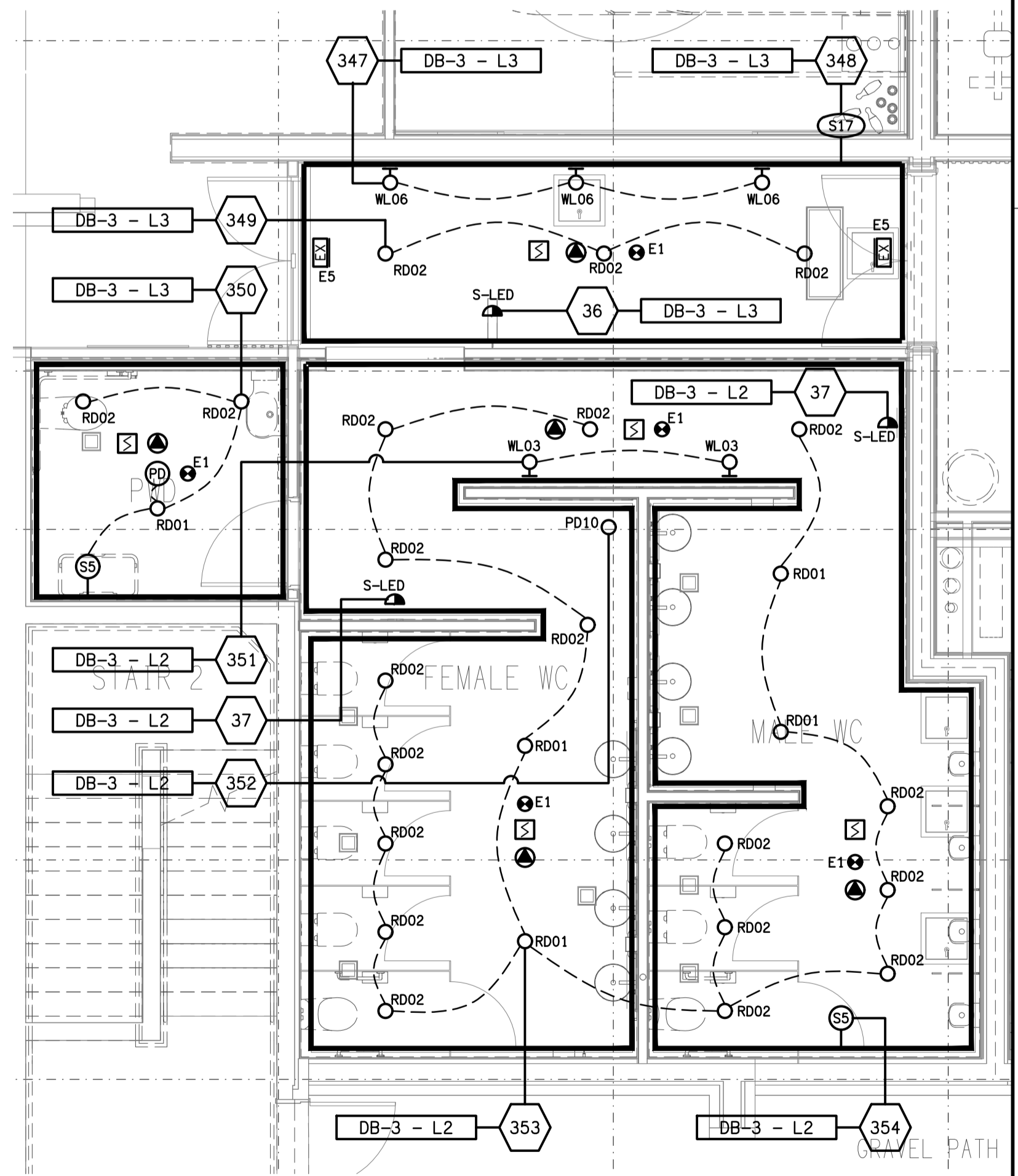
DETAIL A AMENITIES REFLECTED CEILING PLAN SCALE 1:50
